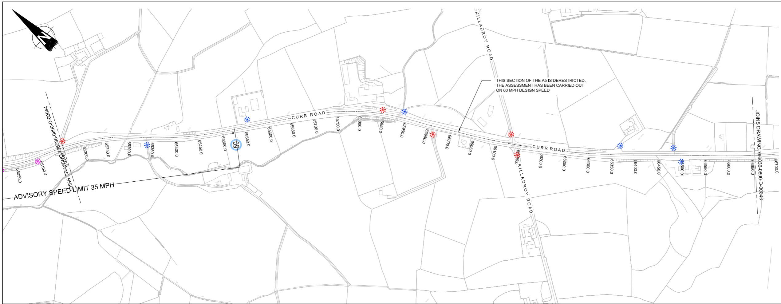
PLAN
